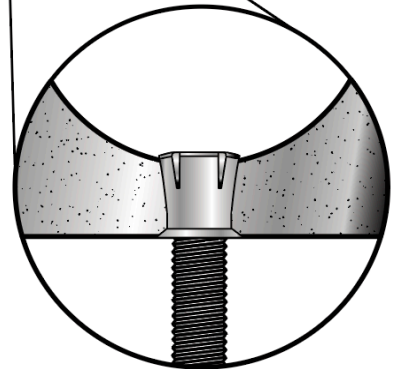
Overhead Core-slab
