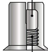
UNC 3/8-16 thread
